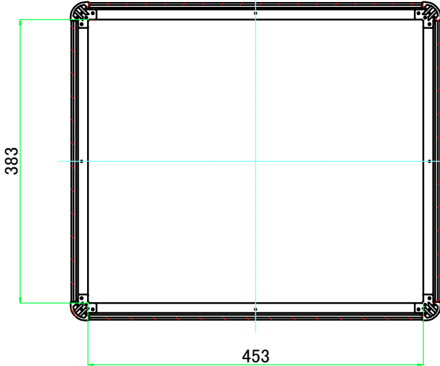
C-C (1:7)
